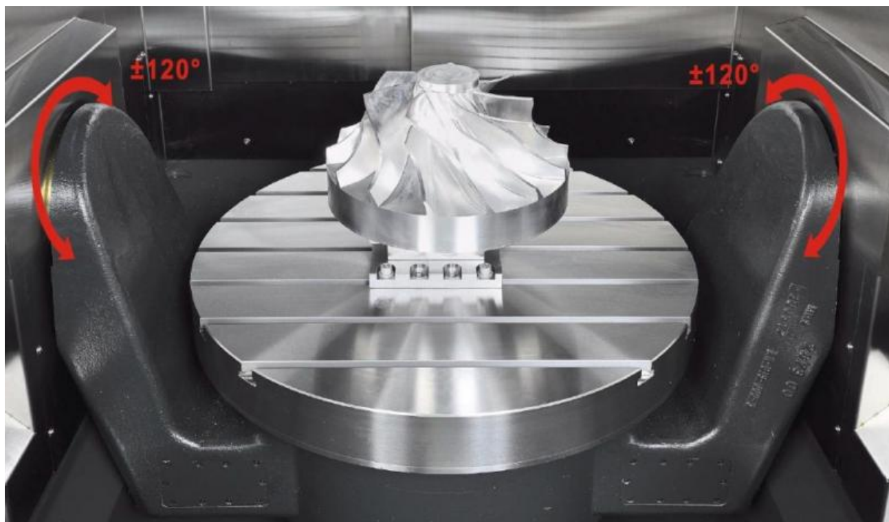
Tavola roto-tiltante Made in Germany
